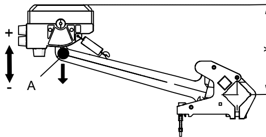
Illustration of the lateral tolerance and contact force 081209
