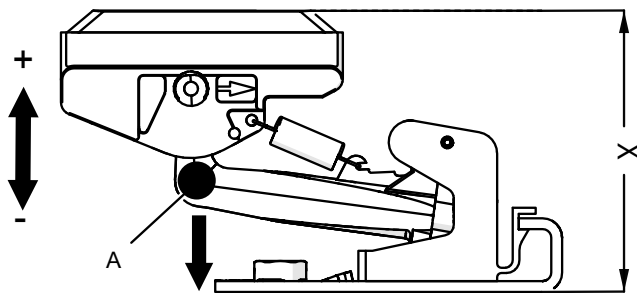
Illustration of the installation distance
